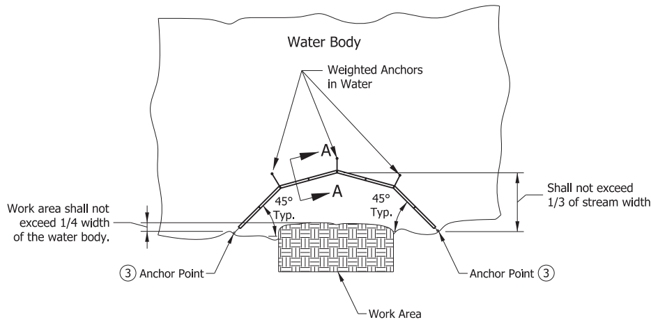
PLAN VIEW ②
